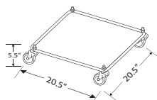
Bola, 4-wheel Dolly R00005
