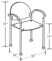
Bola, 4 Leg, Fixed Back, Stacker, with Arms BOL-R44103
